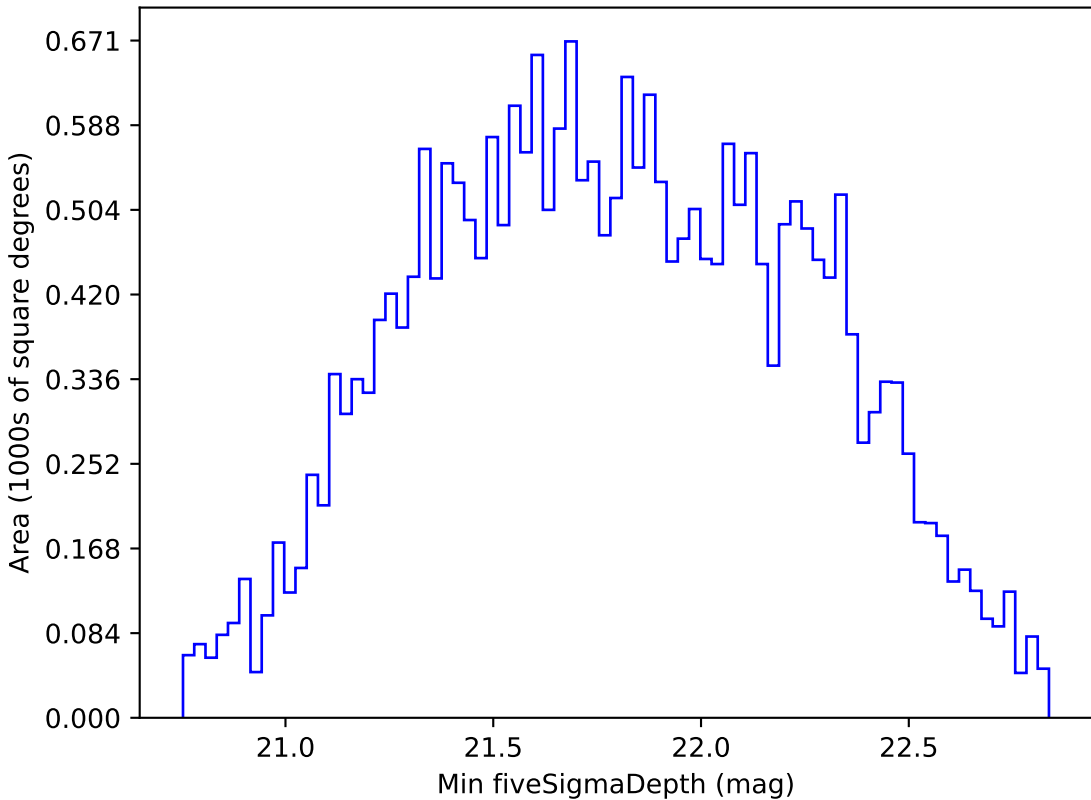
weather_cloudso8v3.4_10yrs All sky i band: Min fiveSigmaDepth
