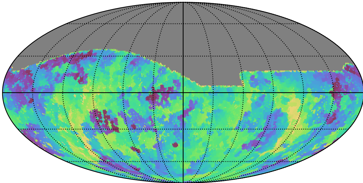
weather_cloudso8v3.4_10yrs All sky g band: Min fiveSigmaDepth
