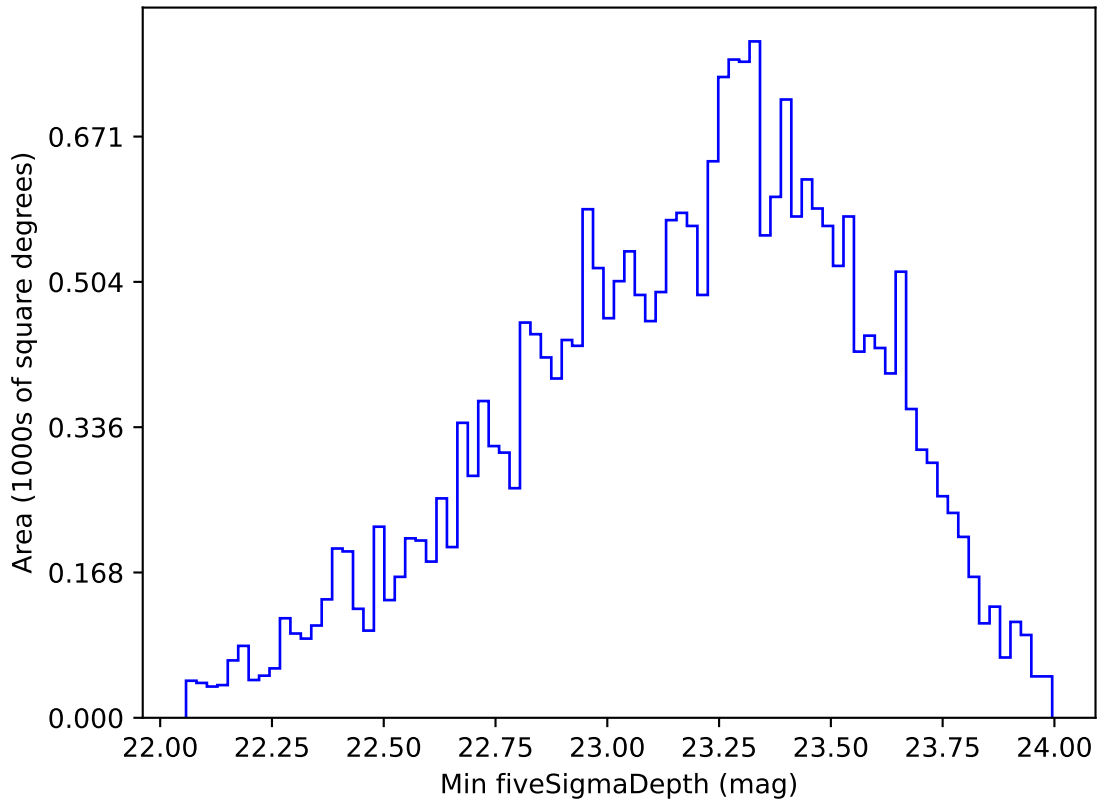
weather_cloudso8v3.4_10yrs All sky g band: Min fiveSigmaDepth
