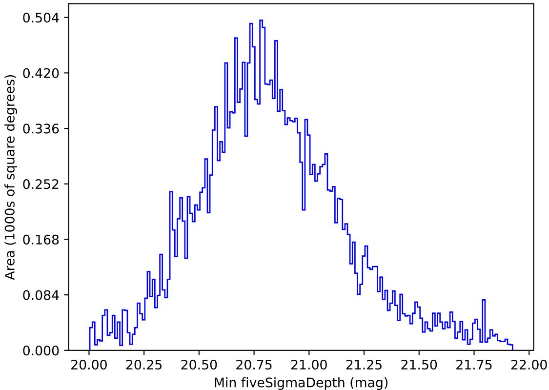
weather_cloudso8v3.4_10yrs All sky all bands: Min fiveSigmaDepth
