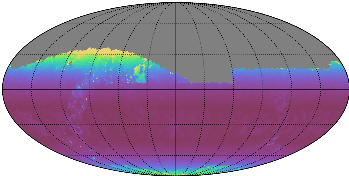
weather_cloudso8v3.4_10yrs Yr 1 z band: Min airmass
