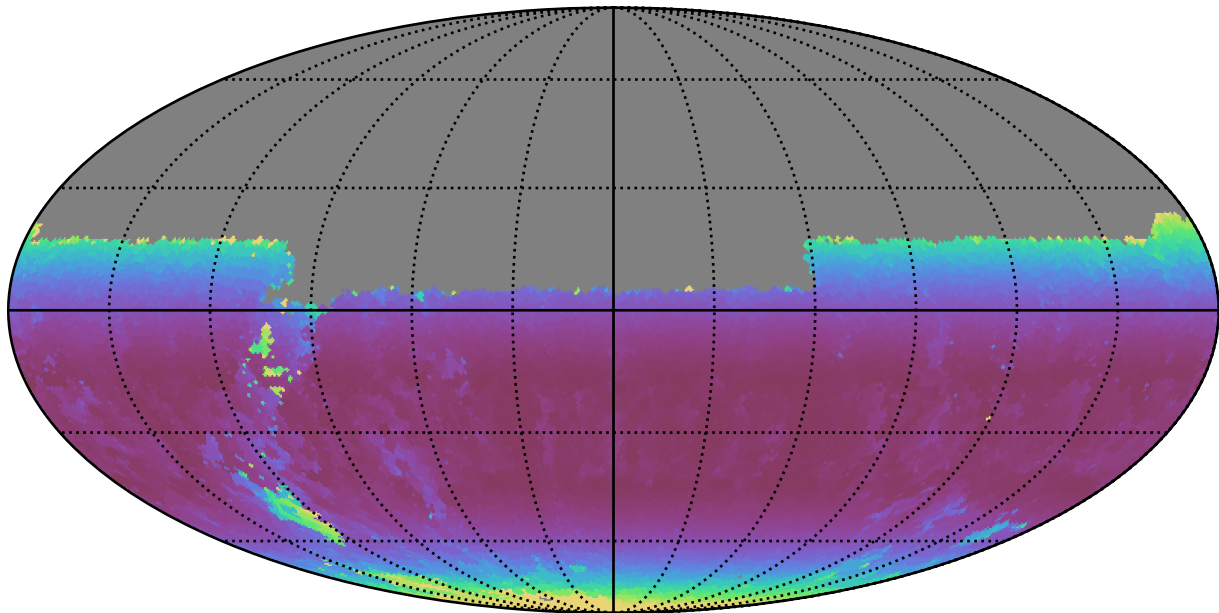
weather_cloudso8v3.4_10yrs Yr 1 y band: Min airmass
