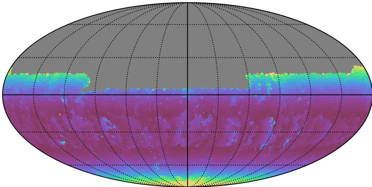
weather_cloudso8v3.4_10yrs Yr 1 u band: Min airmass
