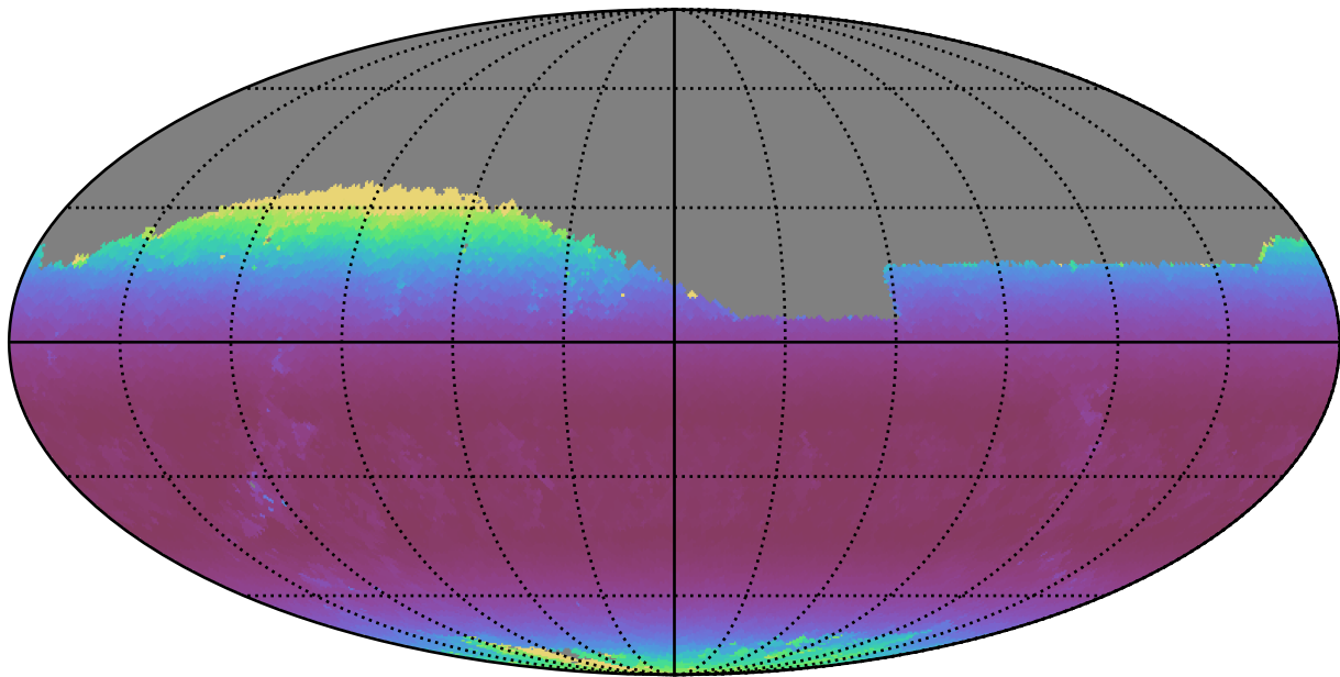
weather_cloudso8v3.4_10yrs Yr 1 r band: Min airmass
