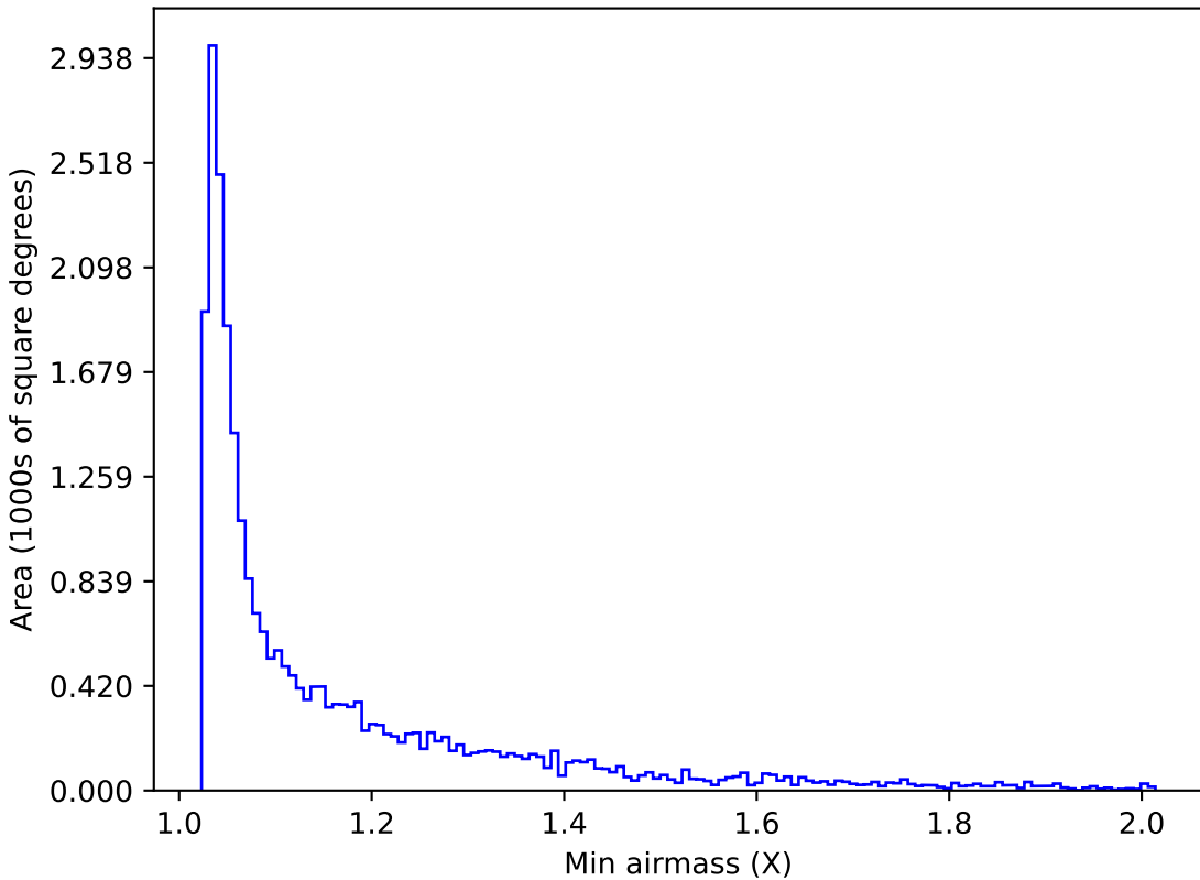
weather_cloudso8v3.4_10yrs Yr 1 r band: Min airmass
