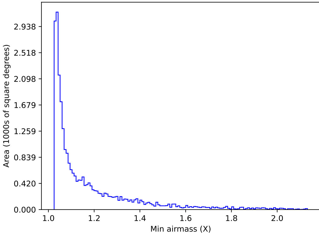
weather_cloudso8v3.4_10yrs Yr 1 i band: Min airmass
