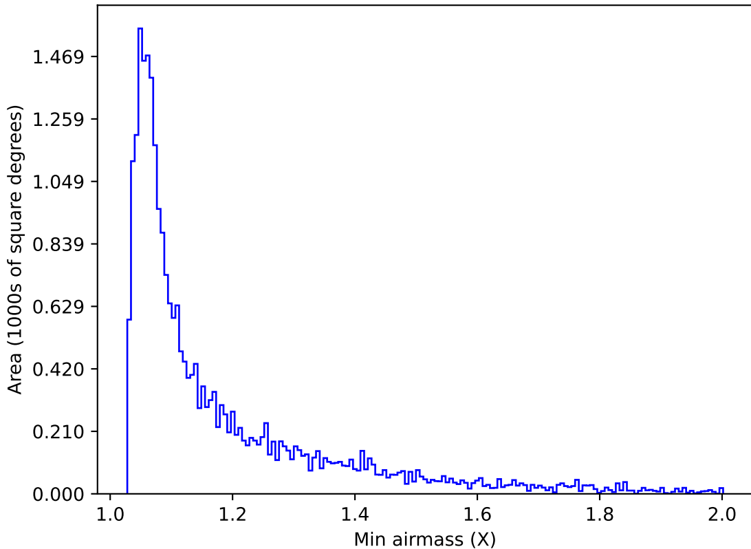
weather_cloudso8v3.4_10yrs Yr 1 g band: Min airmass
