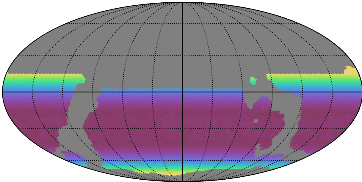
weather_cloudso8v3.4_10yrs WFD z band: Min airmass
