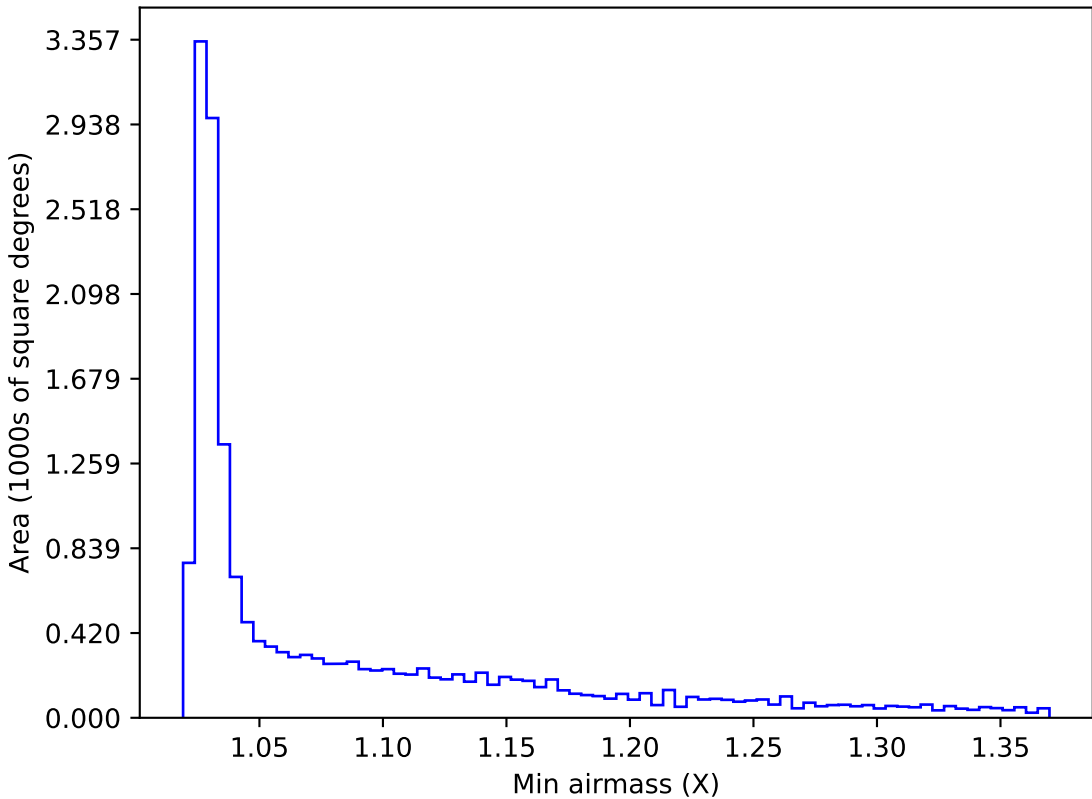
weather_cloudso8v3.4_10yrs WFD z band: Min airmass
