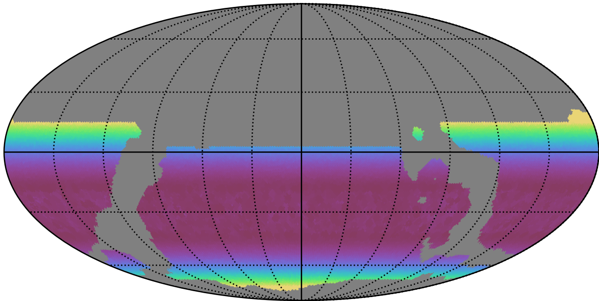
weather_cloudso8v3.4_10yrs WFD y band: Min airmass
