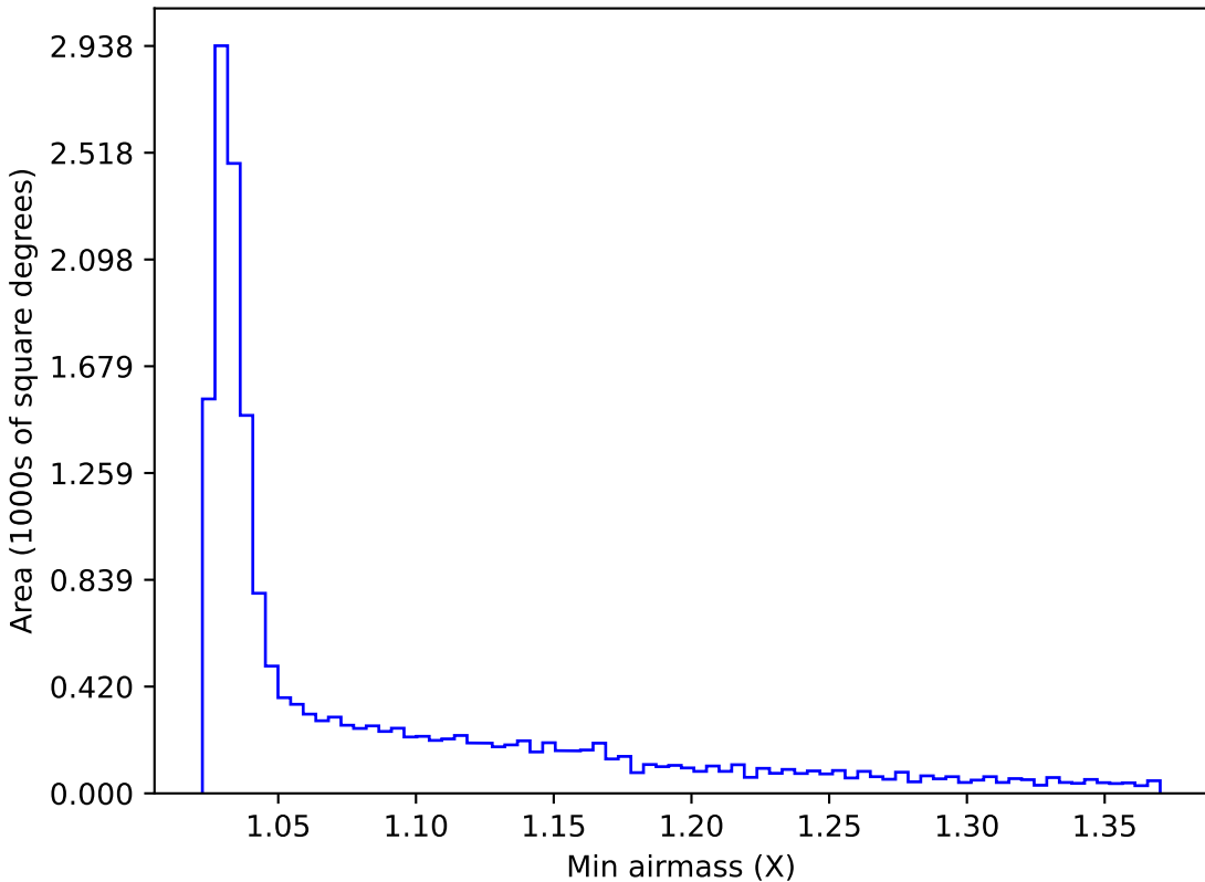
weather_cloudso8v3.4_10yrs WFD y band: Min airmass
