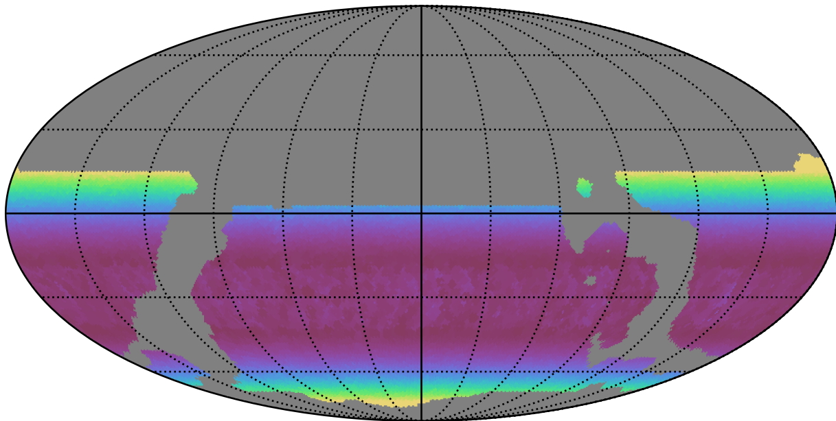
weather_cloudso8v3.4_10yrs WFD u band: Min airmass
