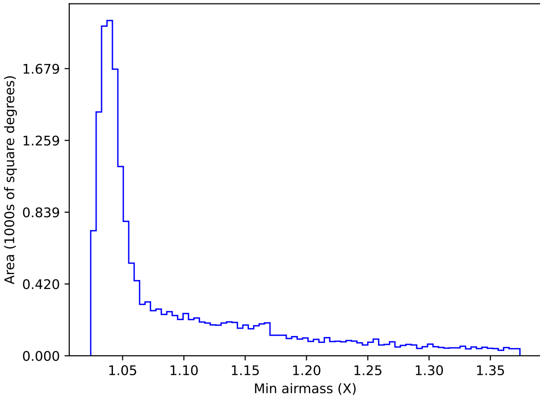
weather_cloudso8v3.4_10yrs WFD u band: Min airmass
