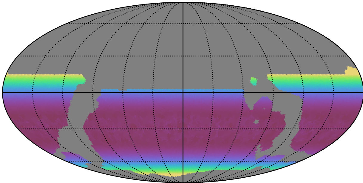
weather_cloudso8v3.4_10yrs WFD r band: Min airmass
