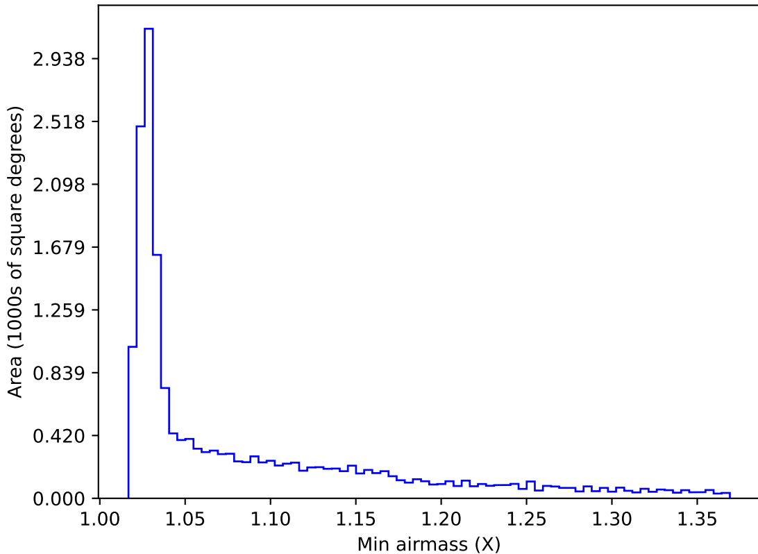
weather_cloudso8v3.4_10yrs WFD r band: Min airmass
