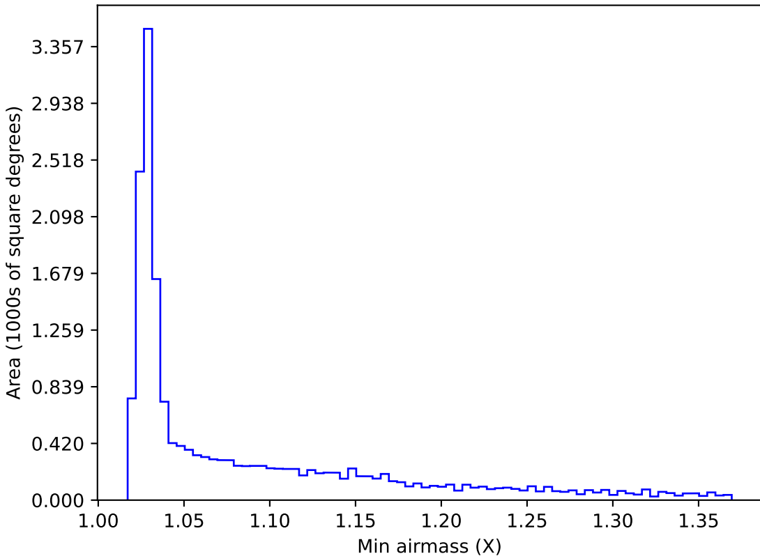
weather_cloudso8v3.4_10yrs WFD i band: Min airmass
