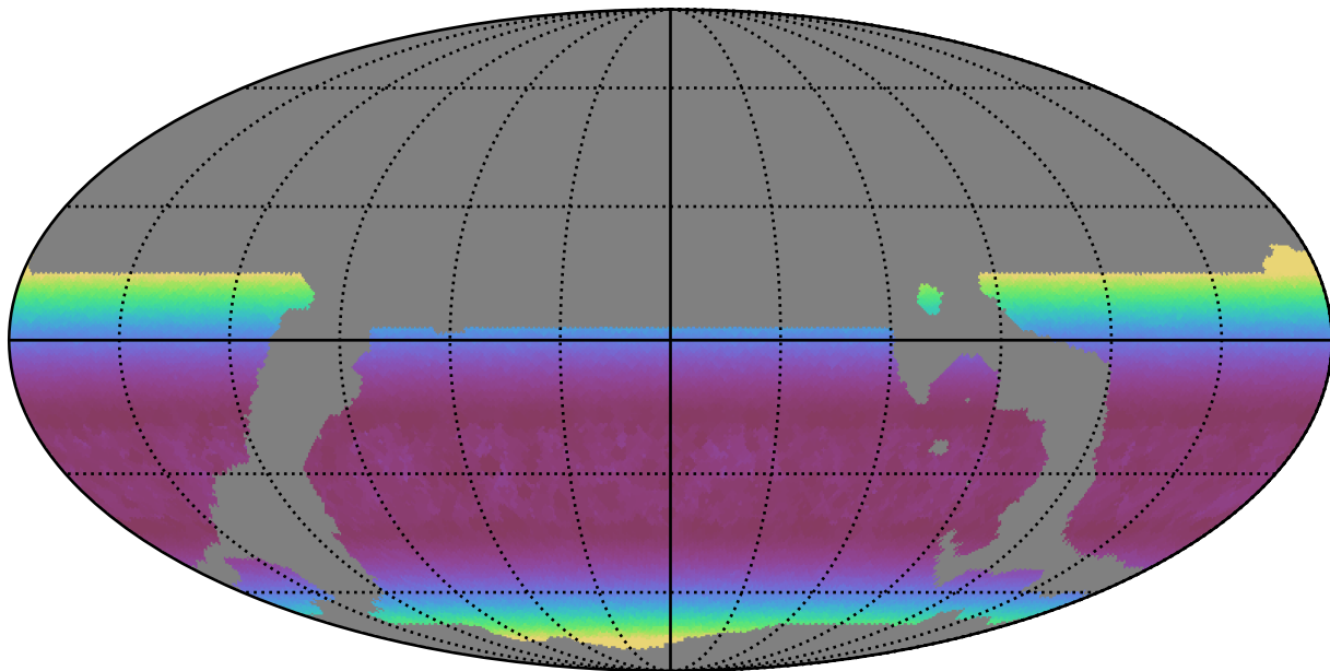
weather_cloudso8v3.4_10yrs WFD g band: Min airmass
