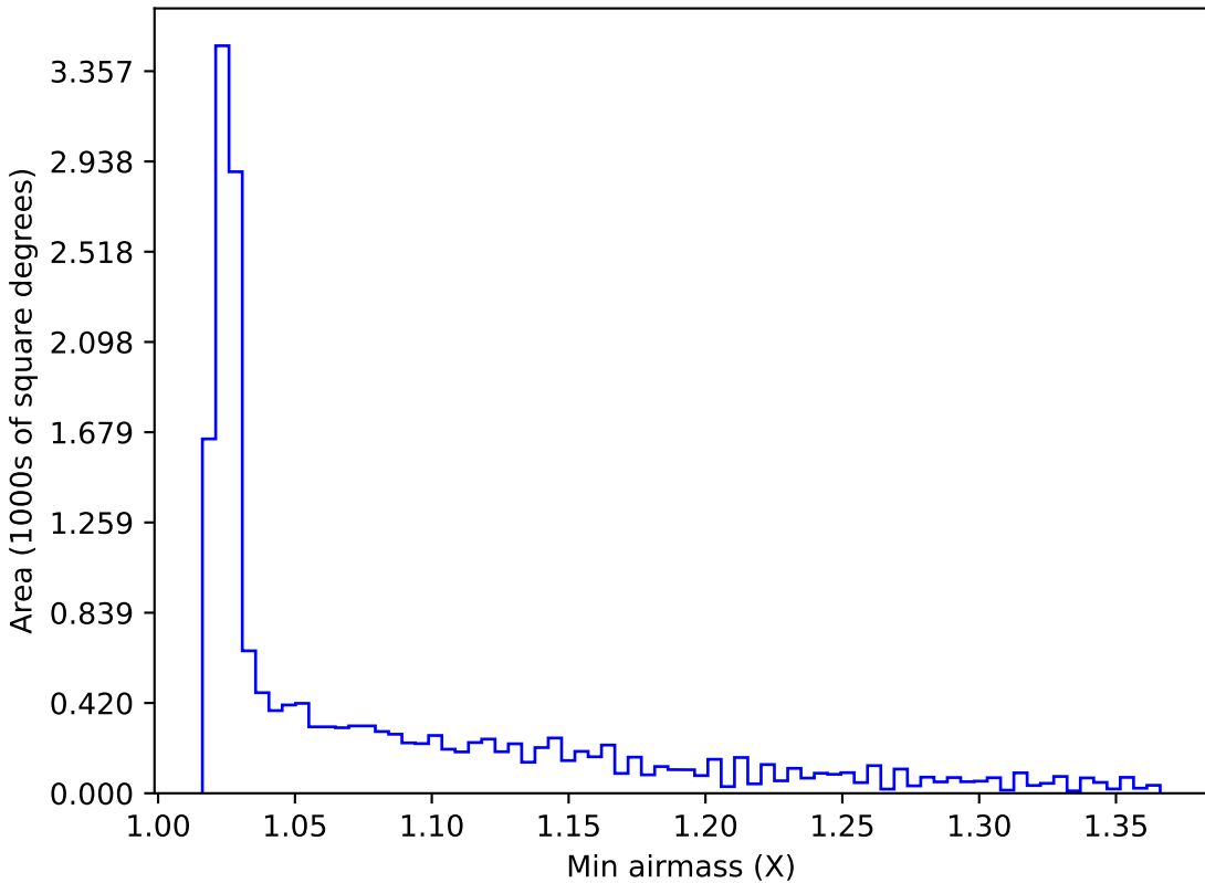
weather_cloudso8v3.4_10yrs WFD all bands: Min airmass
