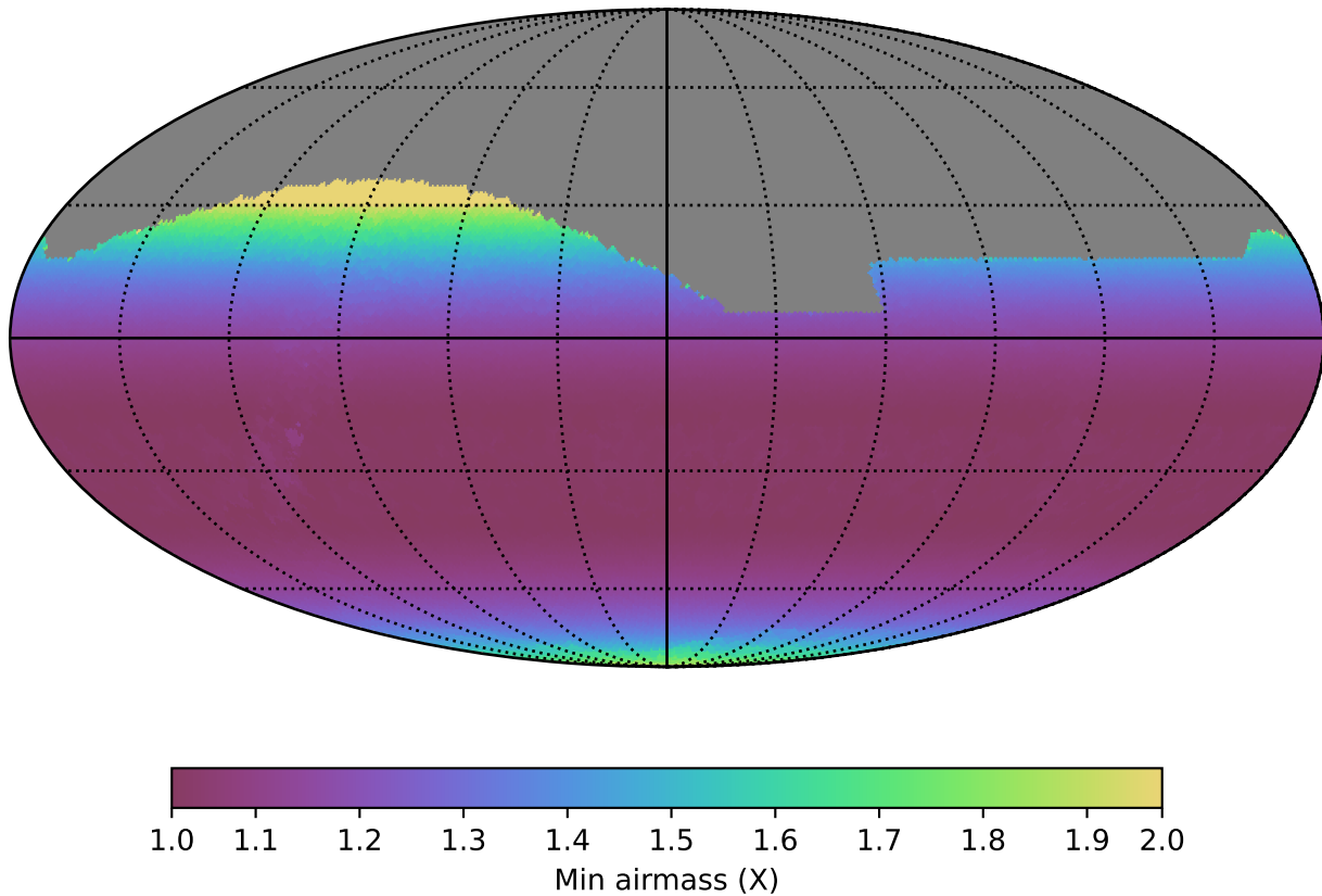
weather_cloudso8v3.4_10yrs All sky z band: Min airmass
