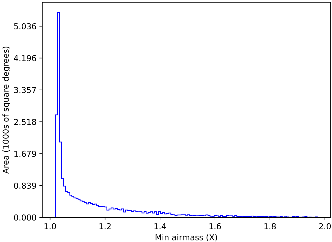
weather_cloudso8v3.4_10yrs All sky z band: Min airmass
