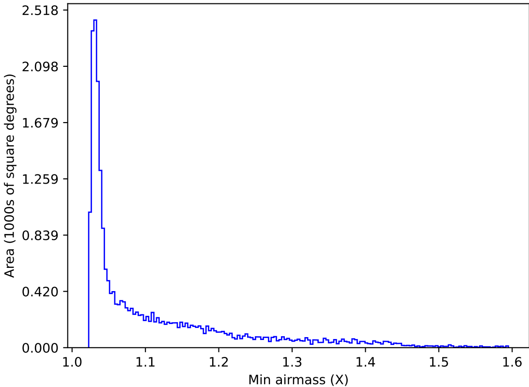
weather_cloudso8v3.4_10yrs All sky y band: Min airmass
