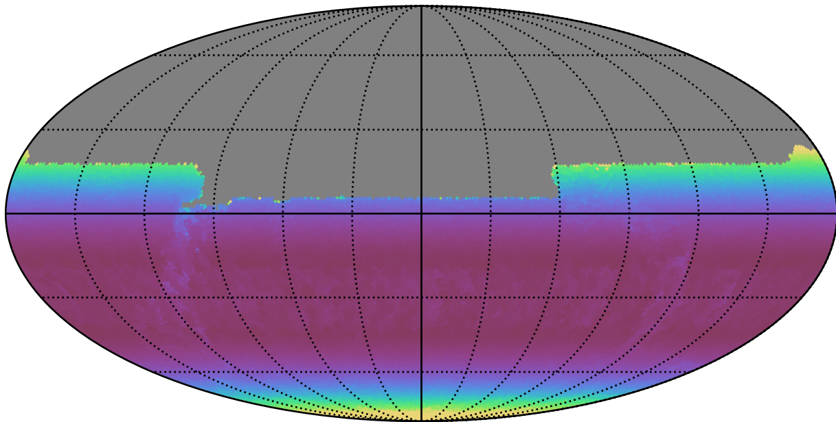
weather_cloudso8v3.4_10yrs All sky u band: Min airmass
