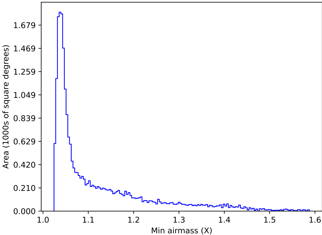
weather_cloudso8v3.4_10yrs All sky u band: Min airmass
