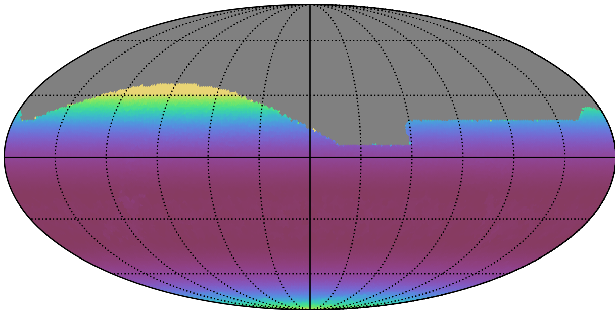
weather_cloudso8v3.4_10yrs All sky r band: Min airmass
