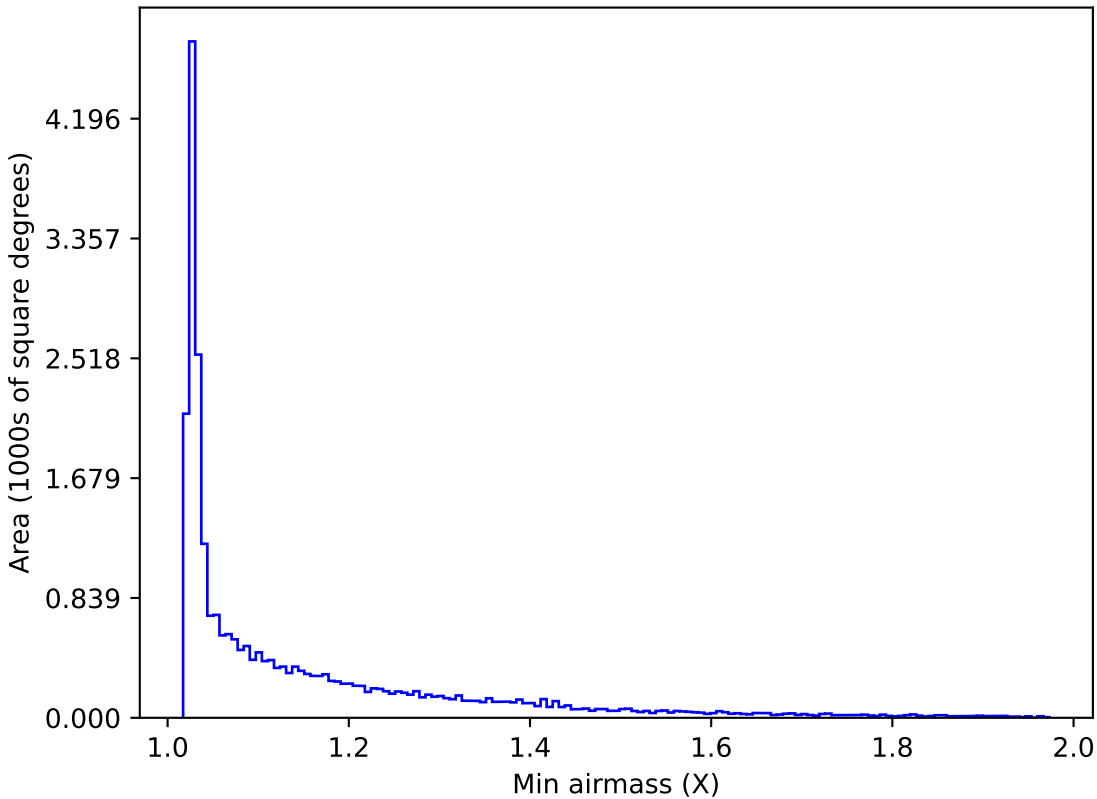
weather_cloudso8v3.4_10yrs All sky r band: Min airmass
