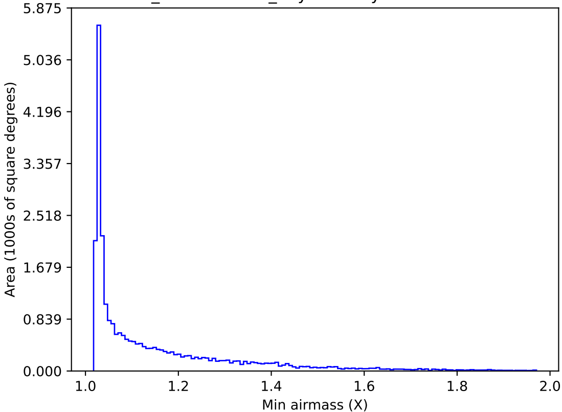
weather_cloudso8v3.4_10yrs All sky i band: Min airmass
