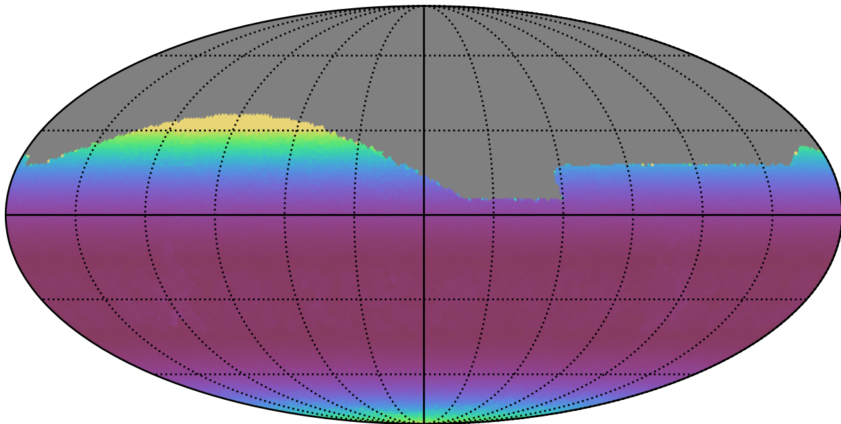
weather_cloudso8v3.4_10yrs All sky g band: Min airmass
