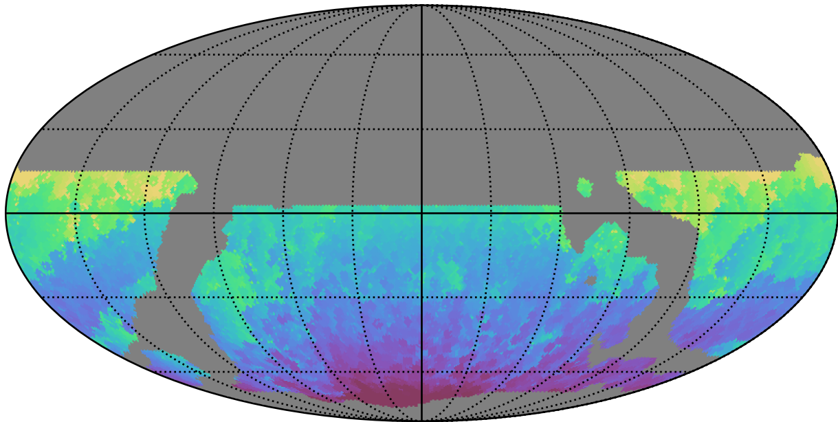
weather_cloudso8v3.4_10yrs WFD z band: Min HA
