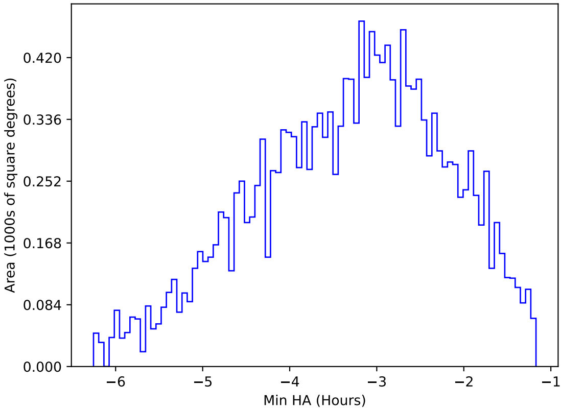
weather_cloudso8v3.4_10yrs WFD u band: Min HA
