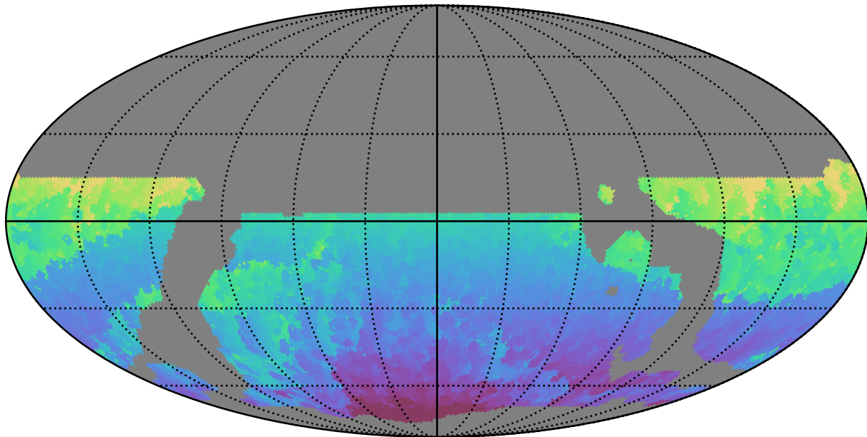
weather_cloudso8v3.4_10yrs WFD r band: Min HA
