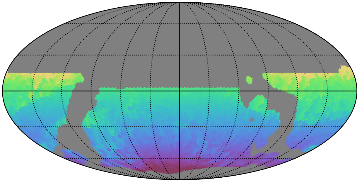
weather_cloudso8v3.4_10yrs WFD all bands: Min HA
