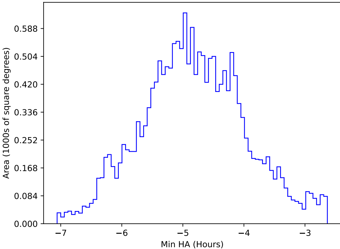
weather_cloudso8v3.4_10yrs WFD all bands: Min HA
