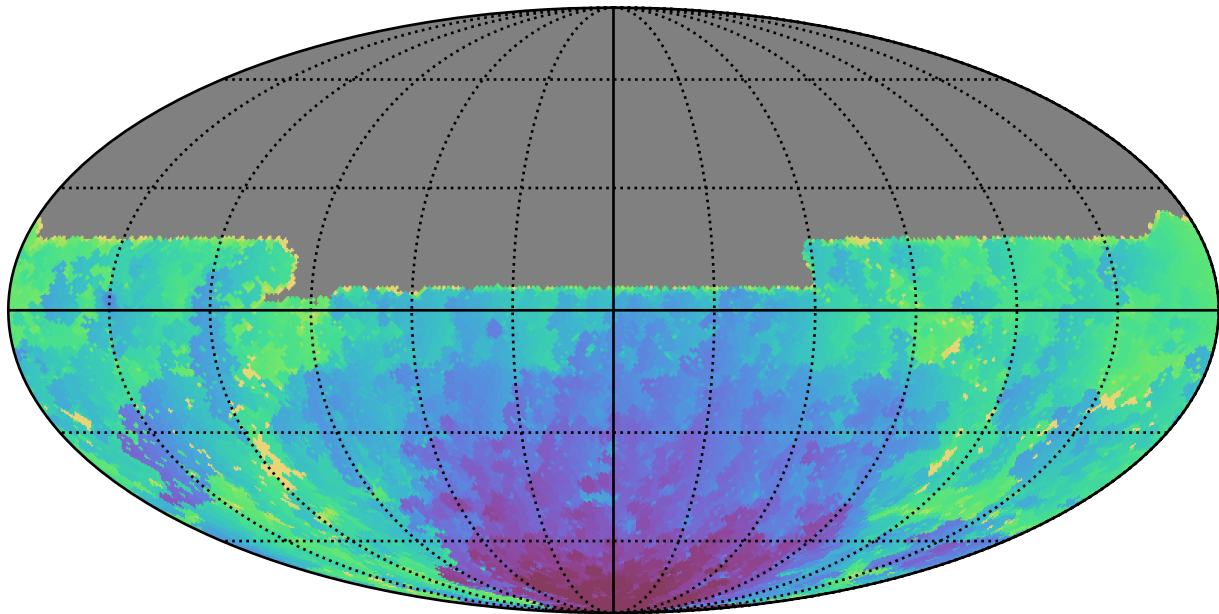
weather_cloudso8v3.4_10yrs All sky u band: Min HA
