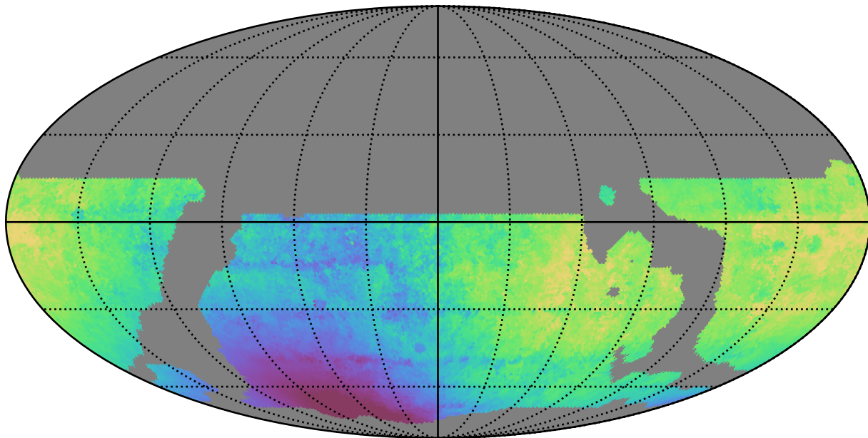
weather_cloudso8v3.4_10yrs WFD z band: Median solarElong
