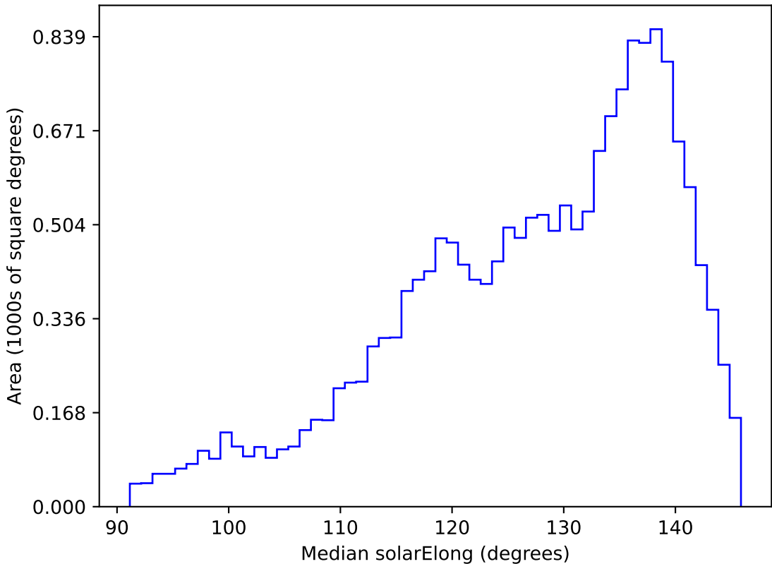
weather_cloudso8v3.4_10yrs WFD z band: Median solarElong
