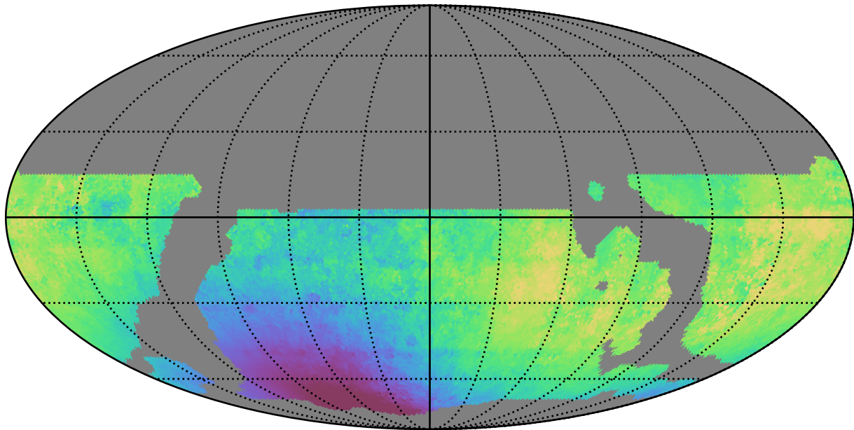
weather_cloudso8v3.4_10yrs WFD y band: Median solarElong
