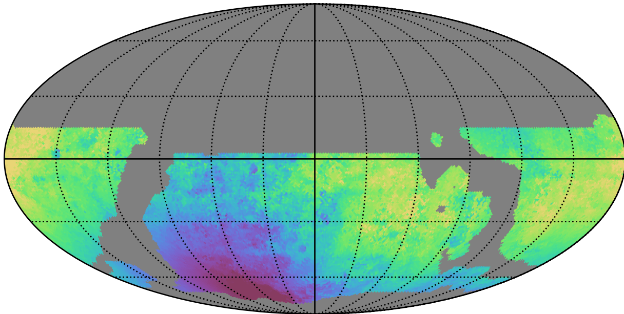
weather_cloudso8v3.4_10yrs WFD u band: Median solarElong
