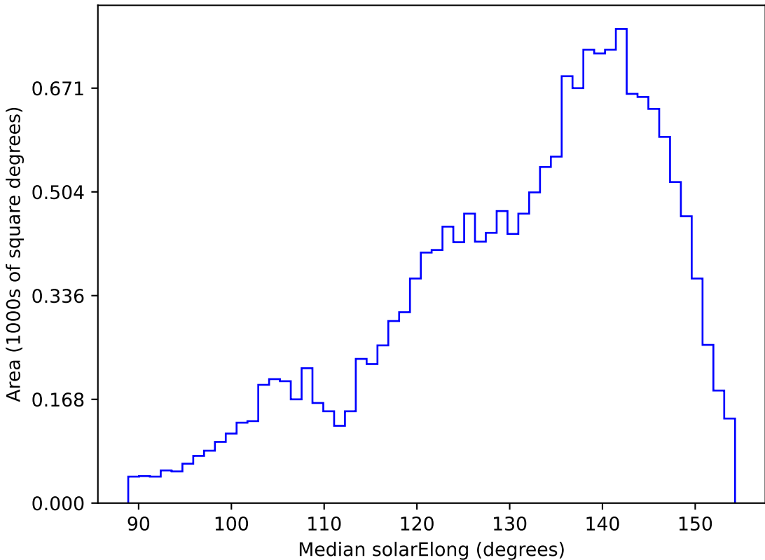
weather_cloudso8v3.4_10yrs WFD u band: Median solarElong
