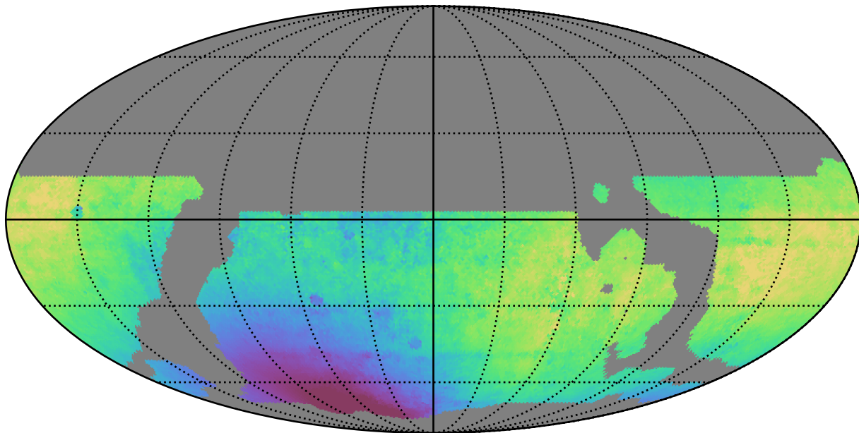
weather_cloudso8v3.4_10yrs WFD r band: Median solarElong
