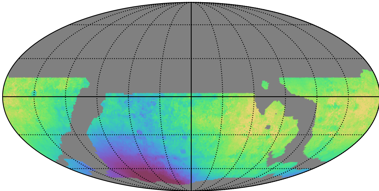
weather_cloudso8v3.4_10yrs WFD i band: Median solarElong
