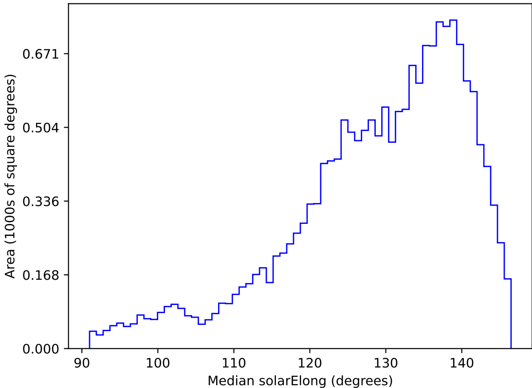
weather_cloudso8v3.4_10yrs WFD i band: Median solarElong
