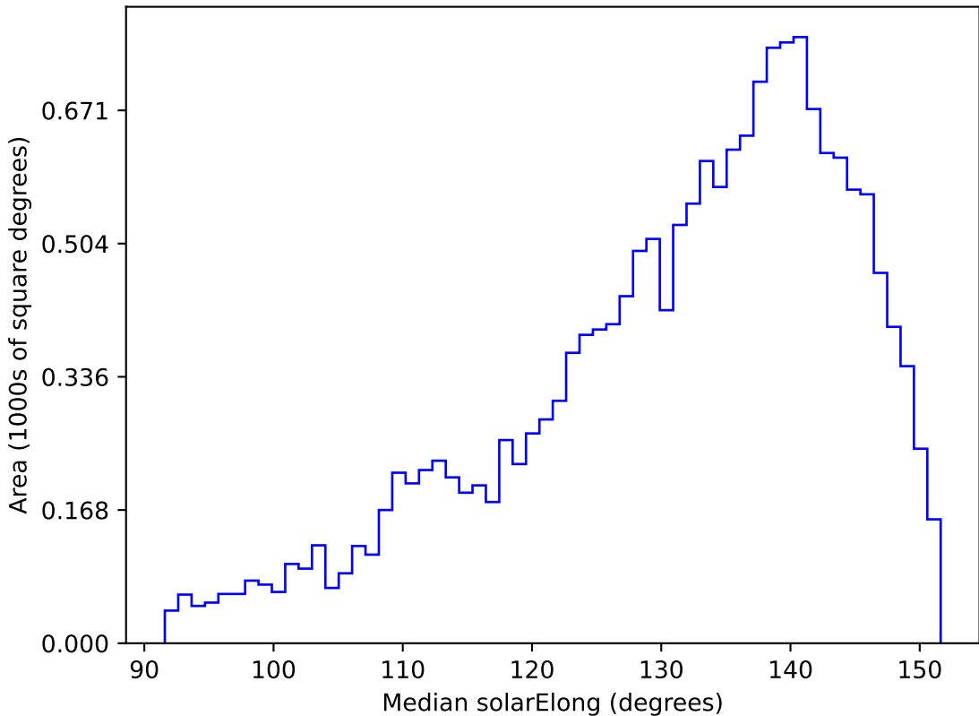
weather_cloudso8v3.4_10yrs WFD g band: Median solarElong
