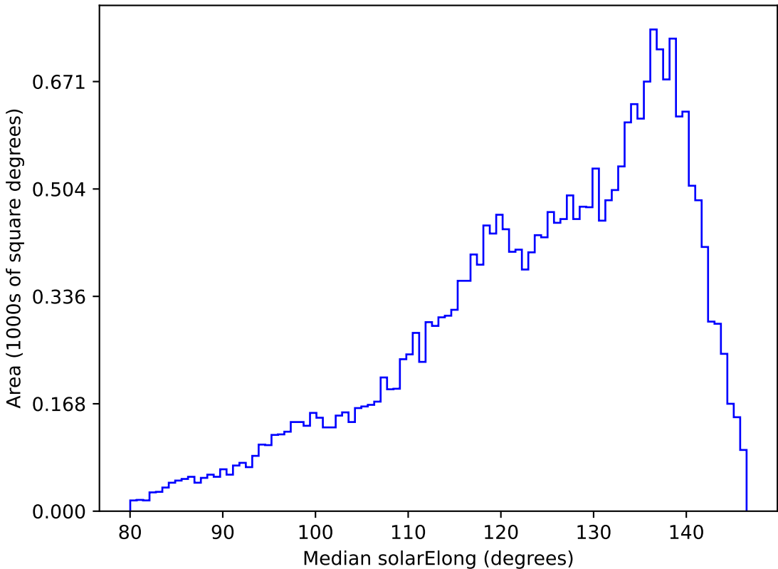
weather_cloudso8v3.4_10yrs All sky z band: Median solarElong
