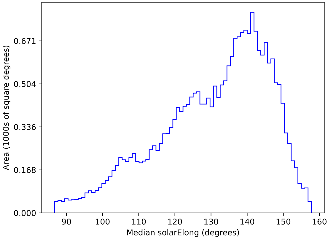
weather_cloudso8v3.4_10yrs All sky u band: Median solarElong
