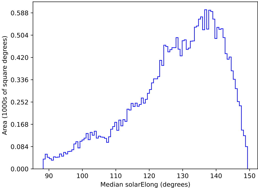
weather_cloudso8v3.4_10yrs All sky r band: Median solarElong
