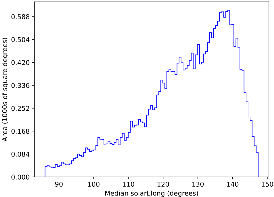
weather_cloudso8v3.4_10yrs All sky i band: Median solarElong
